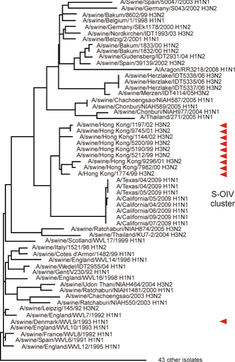
Figure 3 0.05 nucleotide substitutions/site
