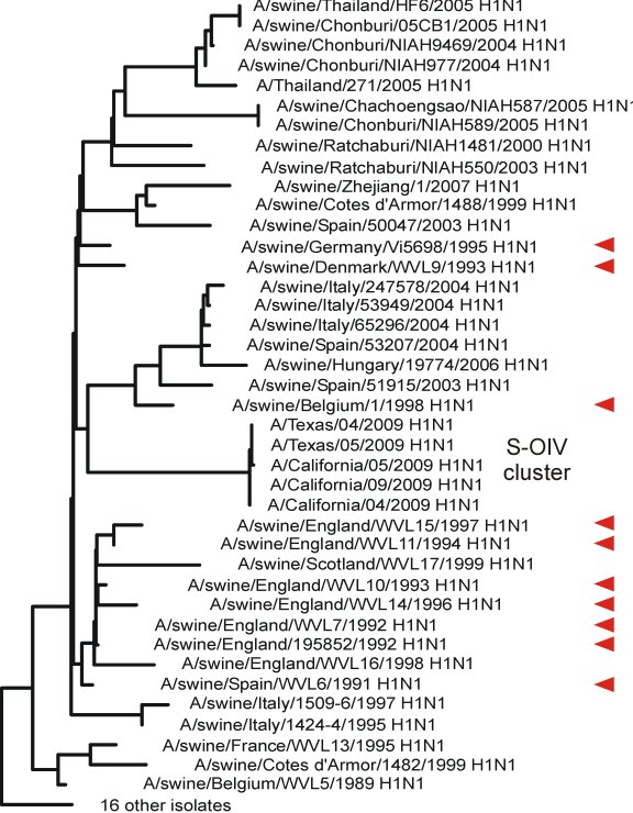
Figure 2 ...nucleotide substitutions/site
